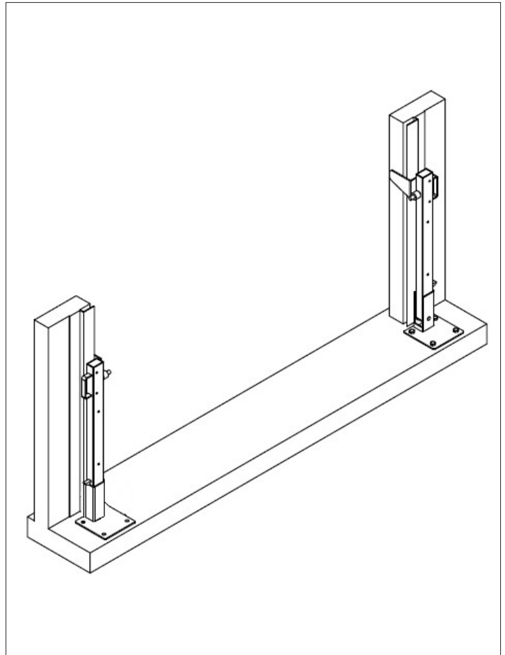
In the open position the left and right gate lock securely into the carriage on either side.
